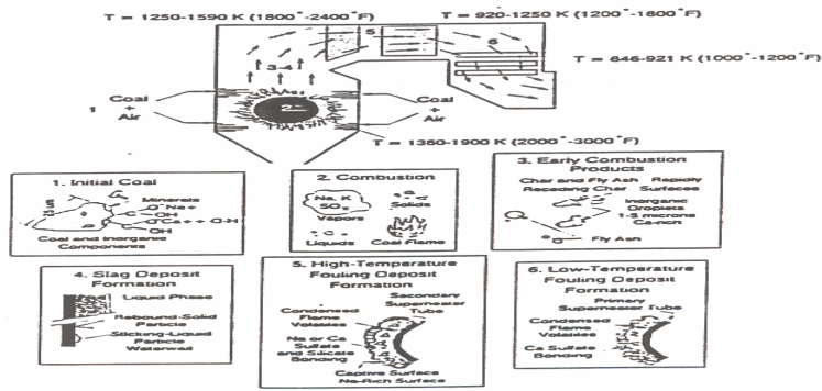
Fig 1. Coal Ash Deposition in Utility Boilers [1].
