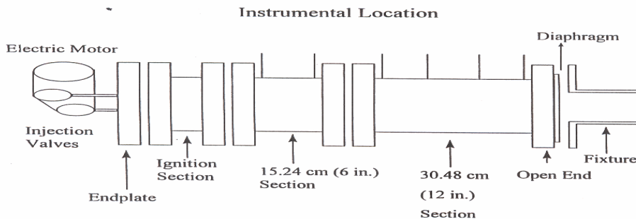
Fig 3. Schematic of the Test Chamber.
