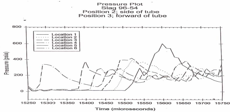
Fig 4. Pressure Plot of Single Pulse Strong Detonation Wave Inside the Detonation Tube
