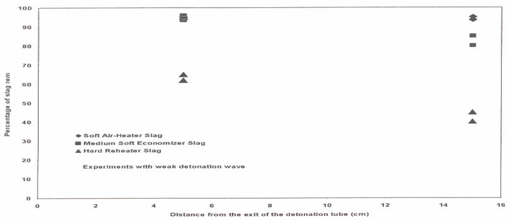
Fig 7. Effect of Slag Type on Slag Removal.
