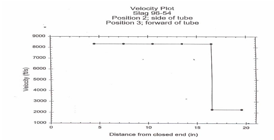
Fig 5. Velocity Plot of Single Pulse Strong Detonation Wave Inside the Detonation Tube
