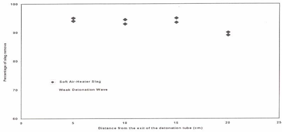
Fig 6. Effect of Axial Positions on Slag Removal
