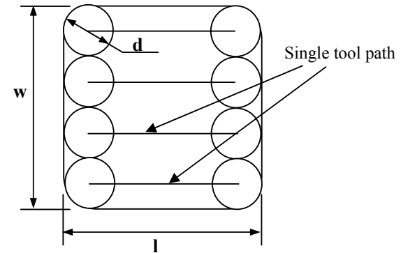
Fig 3: Tool path in zig pattern
