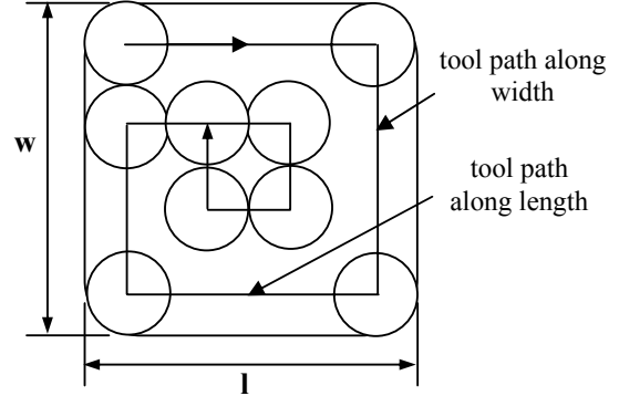
Fig 5: Tool path in spiral-in pattern
