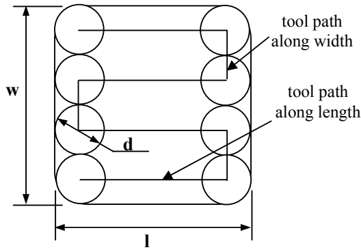
Fig 4: Tool path in zig-zag pattern
