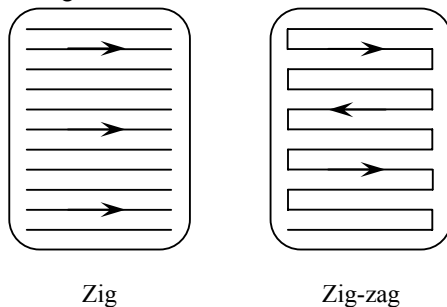
Fi. 1: Direction-parallel tool path pattern
