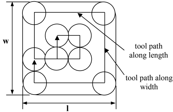
Fig 6: Tool path in spiral-out pattern
