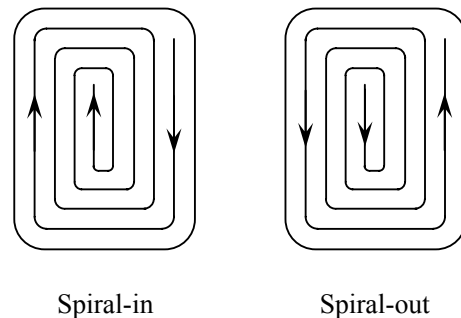
Fig 2: Contour-parallel tool path pattern
