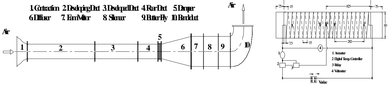
Fig 1: Schematic Diagram of the Experimental Setup
