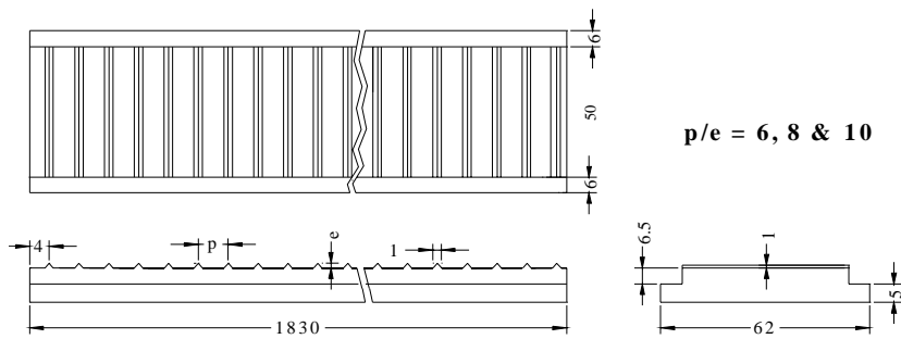
Working Drawing of a Ribbed Wall
