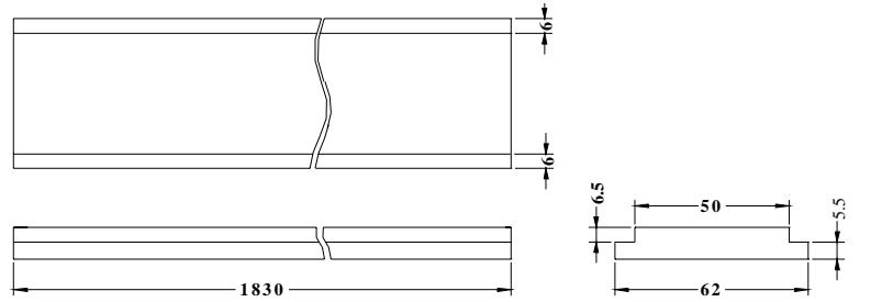
Working Drawing of a Non-Ribbed Wall
