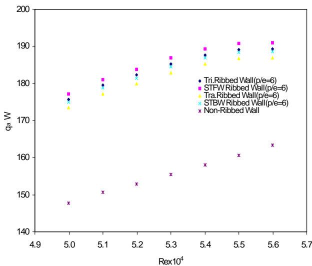
Fig.4 Effect of Reynolds Number on Heat Absorbed of various Types of Ribbed Wall
