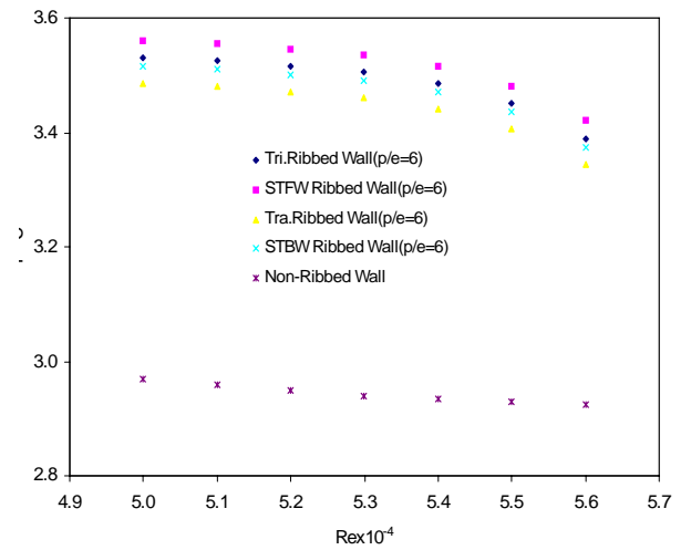
Fig. 7 Effect of Reynolds Number on Temperature Difference various types of ribbed walls.
