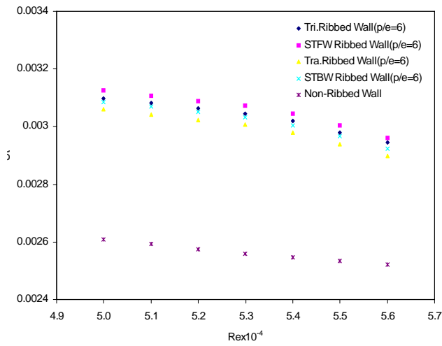
Fig.6 Effect Stanton Number on Reynolds Number of various types of ribbed Wall.
