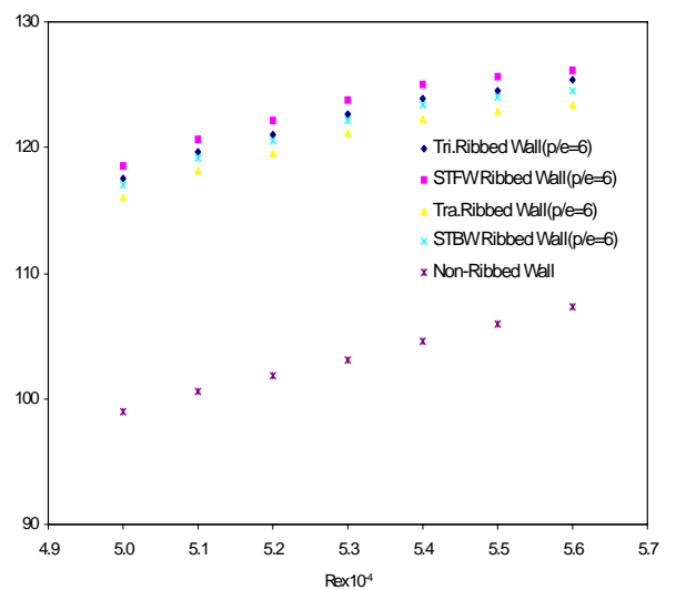
Fig.5 Effect of Nusselt Number on Reynolds Number on various types of Ribbed Wall.
