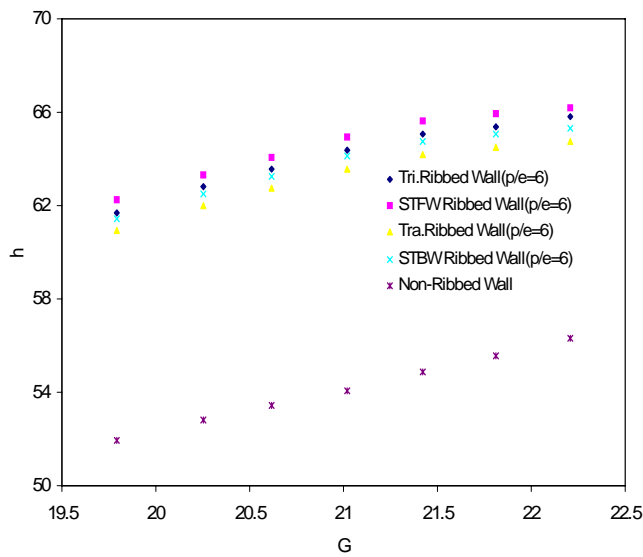
Fig 8 Effect of Mass flux on heat Transfer Co-efficient of various types of Ribbed Wall.
