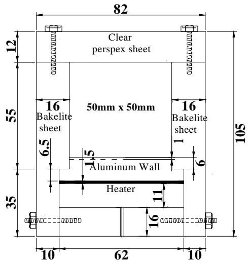
Fig 2: The End View of the Test Duct
