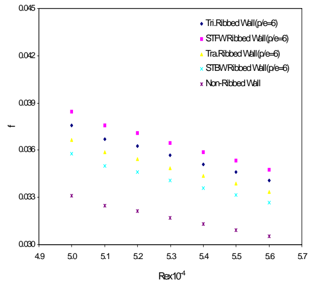
Fig 9 Effect of Friction Factor on Reynolds Number Of various types of Ribbed walls.
