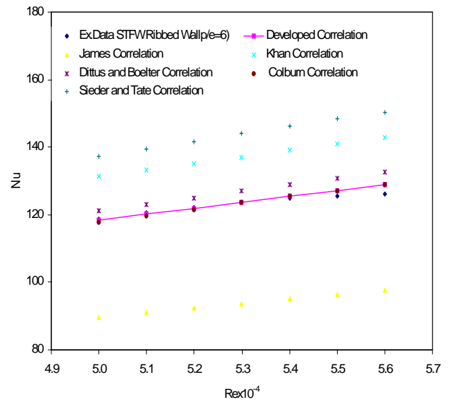
Fig.11 Developed Correlation for Ribbed Ducts in Hydrodynamically Developed Region
