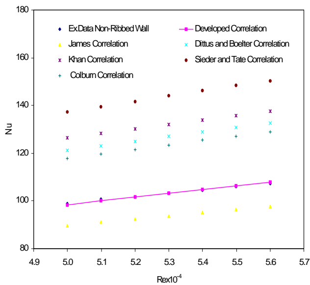
Fig.10 Developed Correlation for Non-Ribbed Ducts in Hydrodynamically Developed Region
